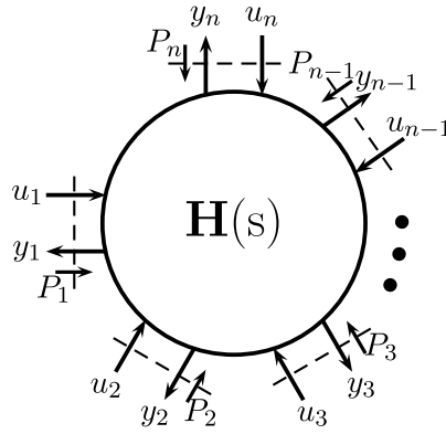
Fig. 2. A linear system \mathbf{H}(s) characterized by n energetic ports.
