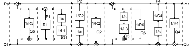
Fig. 21. POG scheme of the hydraulic circuit of Fig. 20.
