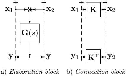
Fig. 1. POG blocks: elaboration block and connection block .
