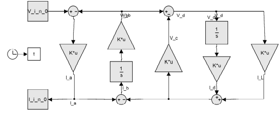
Fig. 16. “SLX, Si” provides the Simulink block scheme.
