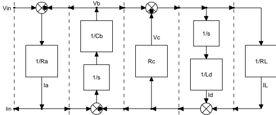
Fig. 15. “POG, Si” provides the POG block scheme.
