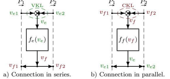
Fig. 5. POG schemes of the series and parallel connections.
