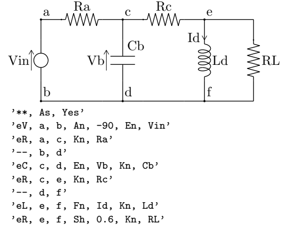
Fig. 13. Electrical example: the physical system and the corresponding “command-lines”.
