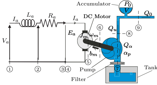
Fig. 7. A DC motor connected to an hydraulic pump.
