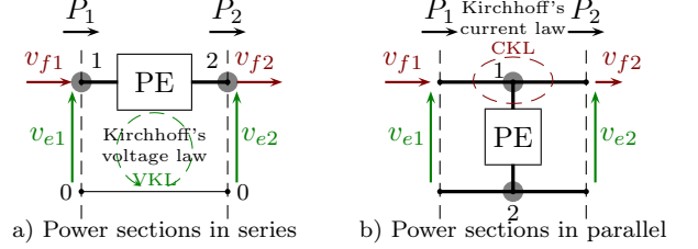
Fig. 4. Connections of the PE with the external world.
