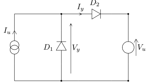
Fig. 1. Electric circuit of the single-phase, half-wave rectifier.
